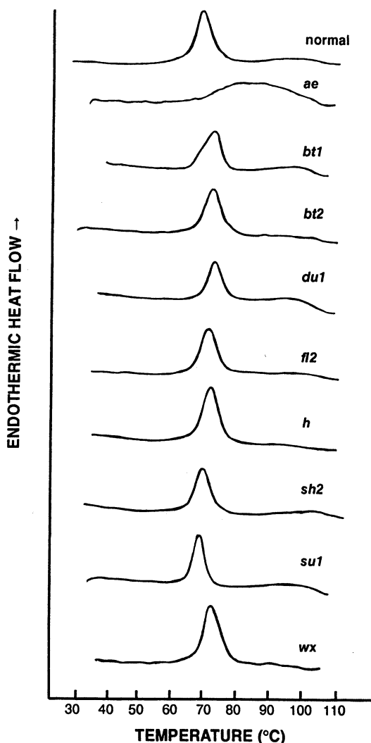
Fig. 2. Differential scanning calorimetry thermograms of single-mutant starches within the Oh43 inbred line.
