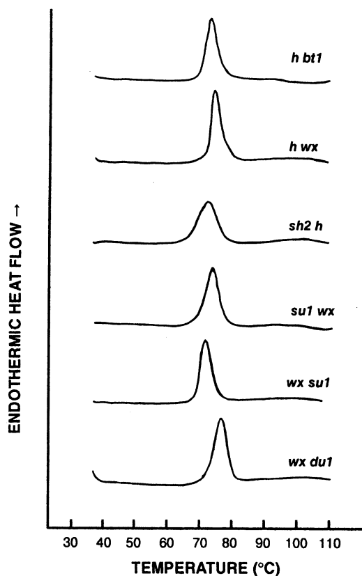
Fig. 3. Differential scanning calorimetry thermograms of selected double-mutant starches within the Oh43 inbred line.
