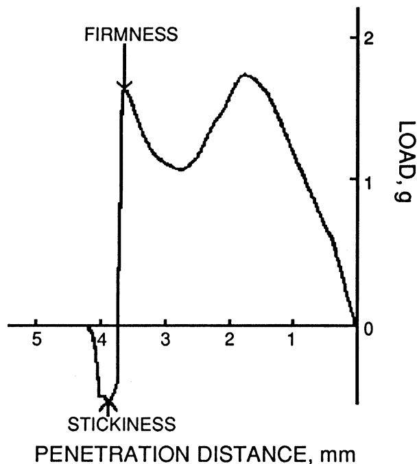
Fig. 1. Load penetration curve of 6% (w/w) commercial corn starch gel measured by the Volland-Stevens texture analyzer. The gel was aged for 4 hr at 25°C before measurement.
